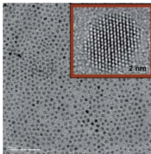
HRTEM image of ZrO 2 nanocrystal processed by solvothermal process
